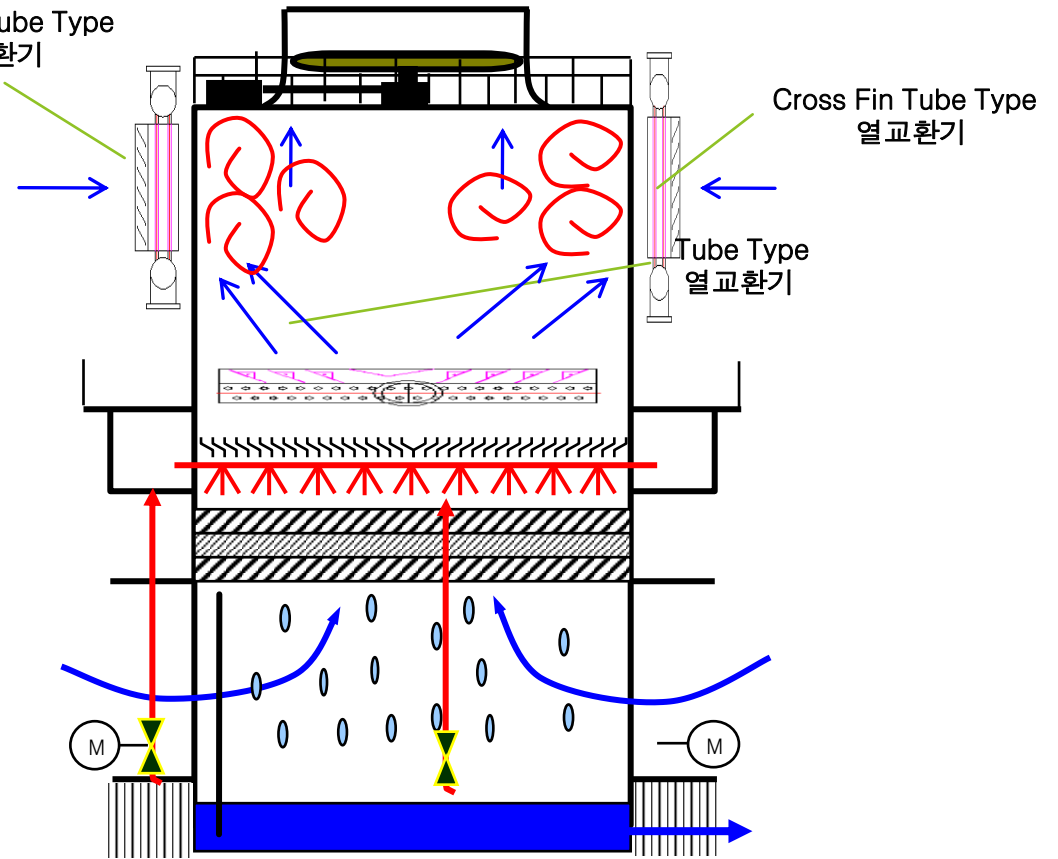
Cooling Tower
